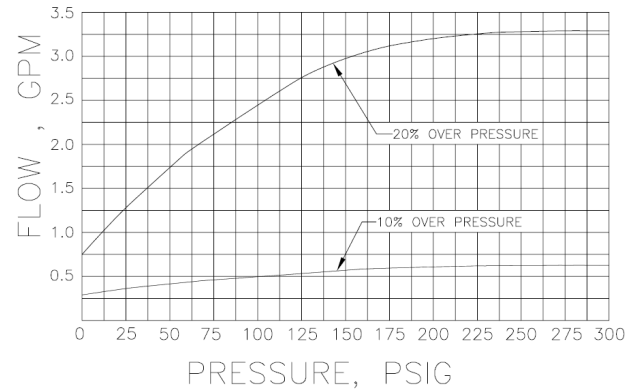
Model 103D-3 Flow Capacity
